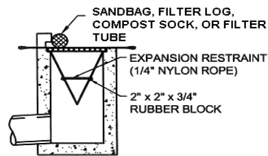
INSTALLATION DETAIL
