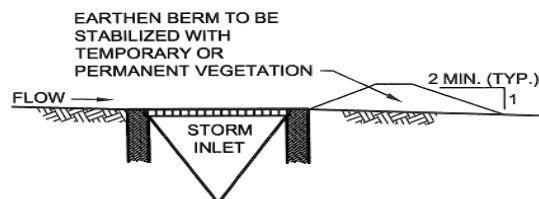
ELEVATION VIEW
