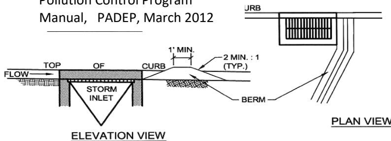
ELEVATION VIEW
