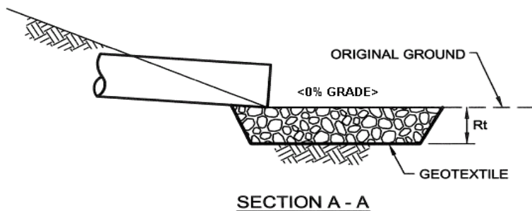
ROCK OUTLET PROTECTION DIAGRAM - From Erosion and Sediment Pollution Control Program Manual, PADEP, March 2012
